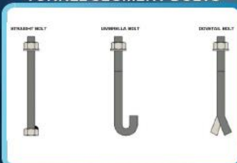
FOUNDATION BOLTS
